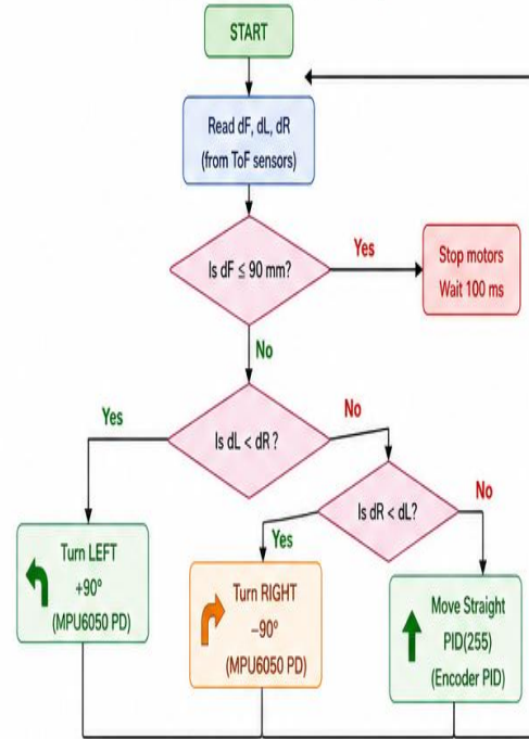
MAIN LOOP DECISION FLOW (Flowchart)
