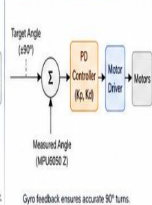
TURN CONTROL (MPU6050 Gyro PD)
