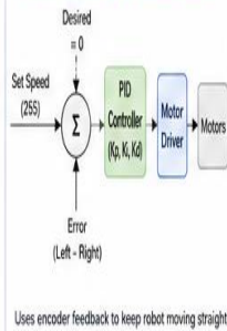
STRAIGHT-LINE PID (Encoder-Based)
