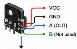
Left Encoder (Wheel)
